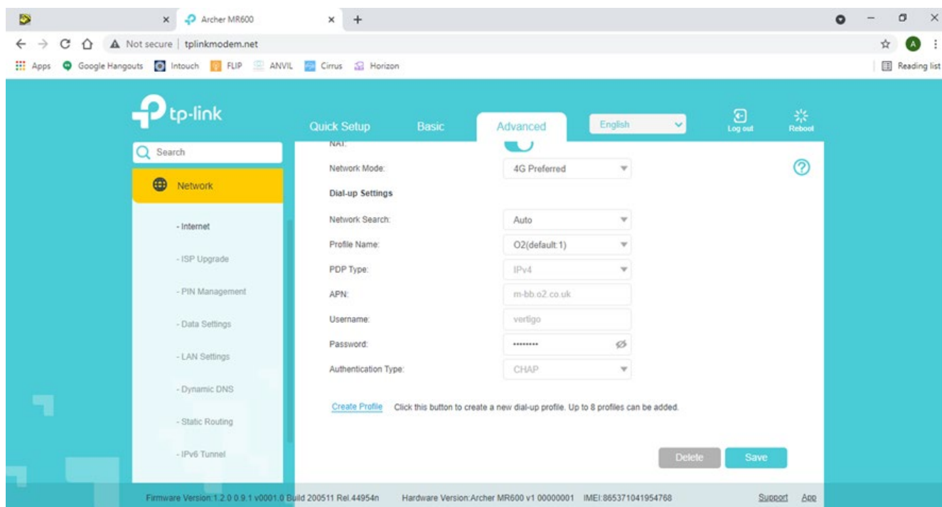
DIAGRAM 3 - CREATING PROFILES
